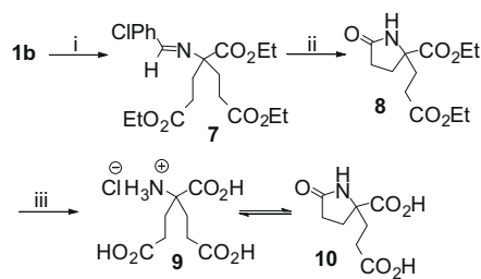
Scheme 2. Synthesis of aminocitrate homolog. Reagents and conditions: (i) \text{K}_2\text{CO}_3 , \text{CH}_2=\text{CHCO}_2\text{Et} , EtOH, rt, 16 h; (ii) 1 N HCl, \text{CH}_3\text{CN} , rt, 30 min, then basic work-up; (iii) 6 N HCl, 120 °C, 24 h.
