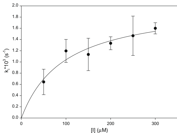
Figure 2. Interaction between 3e and OXA-10. Variation of k_i at 50, 100, 150, 200, 250 and 300 \mu\text{M} in inhibitor.
