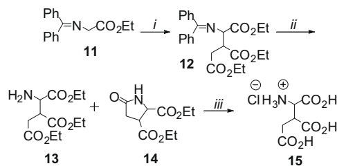
Scheme 3. Synthesis of aminoisocitrate. Reagents and conditions: (i) NaOEt, diethyl fumarate, EtOH, rt, 1 h; (ii) HCl 1 N, \text{CH}_3\text{CN} , rt, 30 min, then basic work-up; (iii) 6 N HCl, 120 °C, 24 h.
