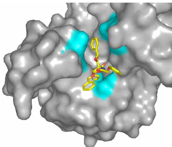
Figure 3. Docking of 4e in OXA-10 enzyme. The hydrophobic residues in the active site are colored in cyan.
