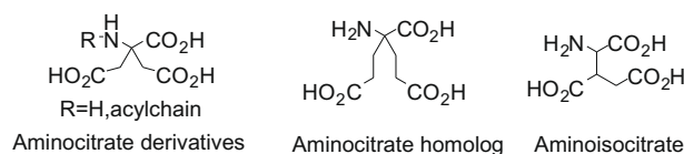
Figure 1. Target molecules (acids and corresponding esters).
