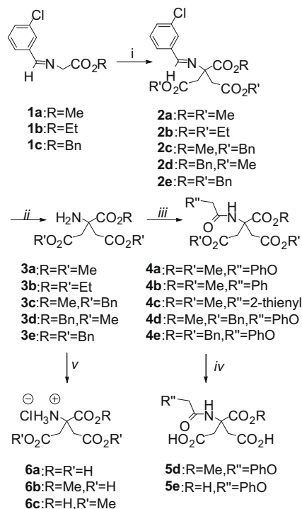
Scheme 1. Synthesis of aminocitrate derivatives. Reagents and conditions: (i) \text{K}_2\text{CO}_3 , \text{Bu}_4\text{NBr} , excess \text{BrCH}_2\text{CO}_2\text{R} , \text{CH}_3\text{CN} , 50 °C or LDA, excess \text{BrCH}_2\text{CO}_2\text{R} , THF, -78 °C to 20 °C; (ii) 1 N HCl, \text{CH}_3\text{CN} , rt, 30 min, then basic work-up; (iv) pyridine, \text{R}''\text{CH}_2\text{COCl} , rt, 5 h; (v) \text{H}_2 , Pd/C, EtOAc, rt, 4 h; (vi) \text{H}_2 , Pd/C, HCl concd, EtOAc, rt, 5 h.
